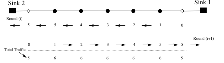
Fig. 5. Two-way traffic dispatching and the amount of traffic forwarded by each node
