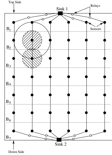
Fig. 4. A novel node deployment with rectangular grid area and 7 Belts
