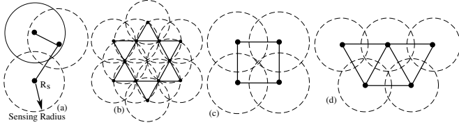
Fig. 1. uniform random (a), a pattern-based Tri-Hexagon Tiling (THT) (b), a Square Grid (c), and Triangle lattice (d) based Coverage
