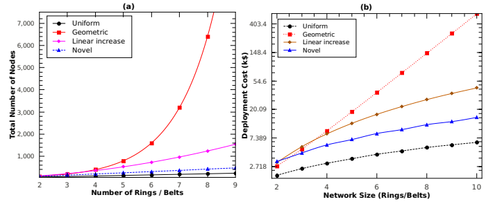
Fig. 7. (a) Total number of deployed nodes when increasing the network size with q = 2 and N_D = 50 . (b) Deployment costs when increasing the network size with q = 2 and N_D = 15
