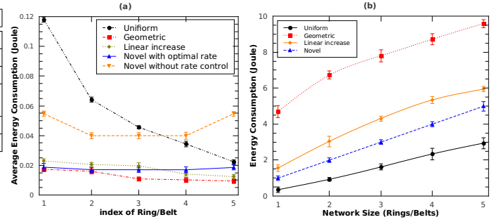
Fig. 8. (a) Average per-node energy consumption in each ring / belt with q = 2 and N_D = 27 . (b) Network energy consumption when increasing the network size.
