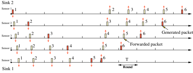
Fig. 6. Optimal data rate r_i^* with required application delay L_{max} = 5T and 5 sensors
