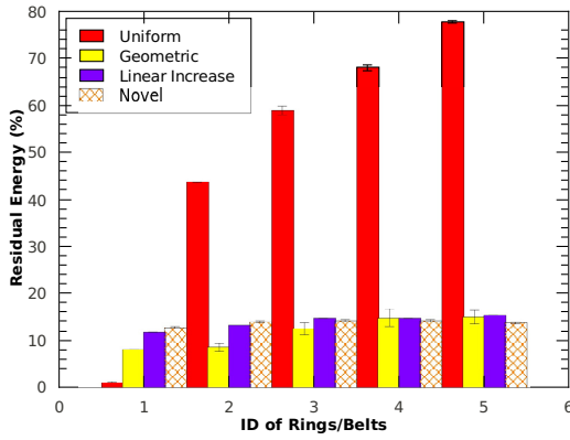
Fig. 9. Residual Energy in each ring or belt when the first node dies with q = 2 , N_D = 27 , and \varepsilon = 0.1 Joules
